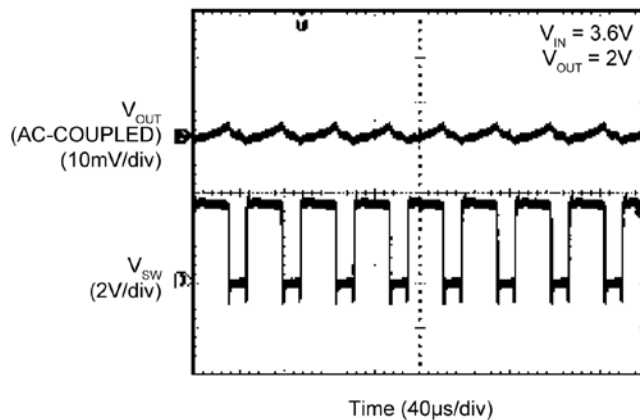
Switching Waveform Continuous Mode (2A)
