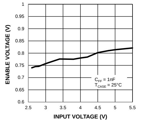
Enable Thresholds vs. Input Voltage
