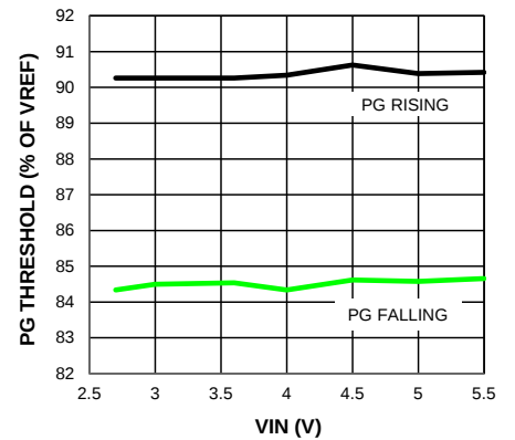
PG Threshold vs. Input Voltage
